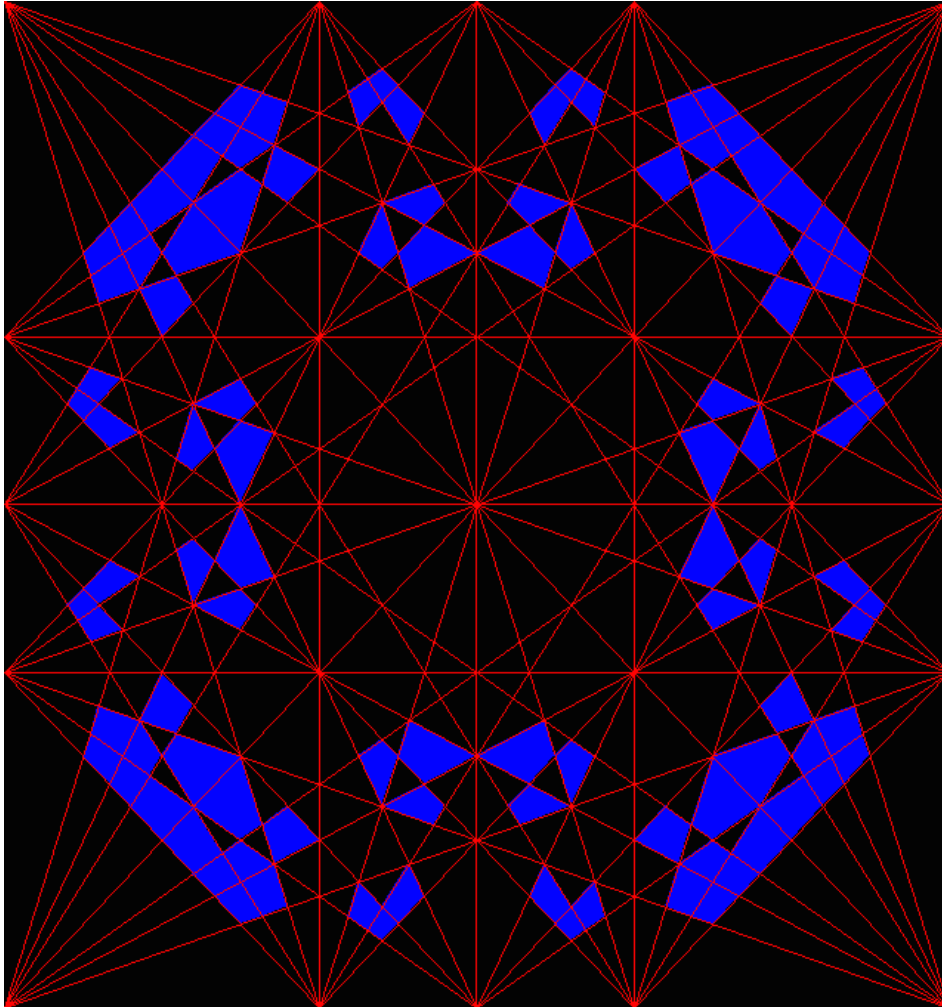
Figure 2: Farey lines of order (3,3)
