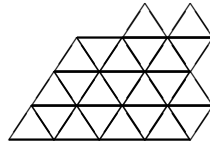
Figure 3: A triangular bargraph
