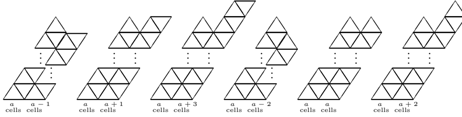
Figure 7: Decomposition of a smooth triangular bargraph such that the first column has type 2 and exactly a cells
