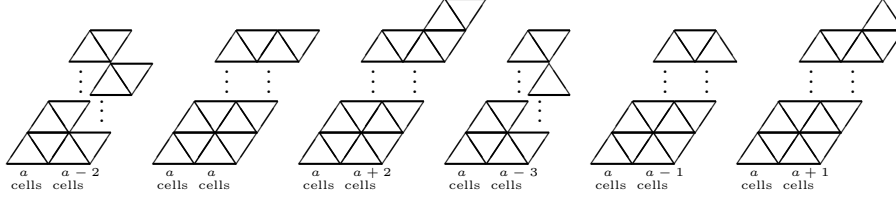
Figure 6: Decomposition of a smooth triangular bargraph such that the first column has type 1 and exactly a cells
