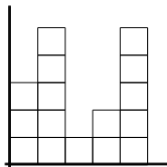
Figure 1: A squared bargraph
