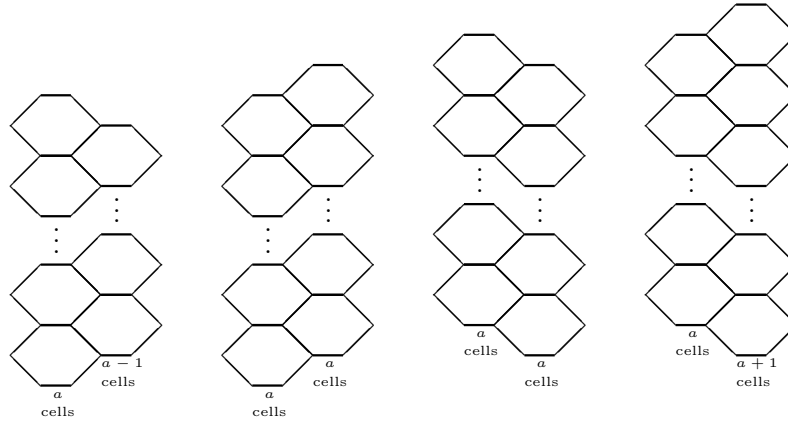
Figure 8: Decomposition of a smooth hexagonal bargraph such that the first column has exactly a cells
