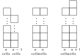
Figure 5: Decomposition of a smooth squared bargraph such that the first column has exactly a cells
