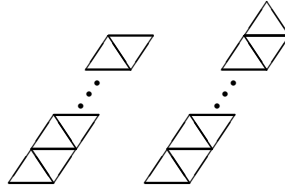
Figure 2: From left to right, columns of type one and two
