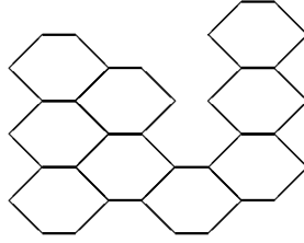
Figure 4: A hexagonal bargraph
