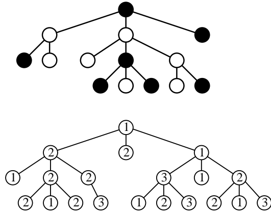
Figure 1. An example of a \bullet_{\circ} -free two-coloured ternary tree of size 14 with a black root and an example of a \circ_{\circ} -free 3-coloured ternary tree of size 20.
