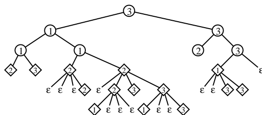
Figure 4. An illustrating example of the bijection presented between a 4-ary tree of size 21 and a \mathcal{O}_{\geq 0} -free 3-coloured binary tree of the same size. The recursive procedure is here performed level by level, where, for better readability, the nodes in the original 4-ary tree are drawn as diamonds. We have omitted the empty subtrees \varepsilon in the original tree as well as for the leaves of the resulting tree.
