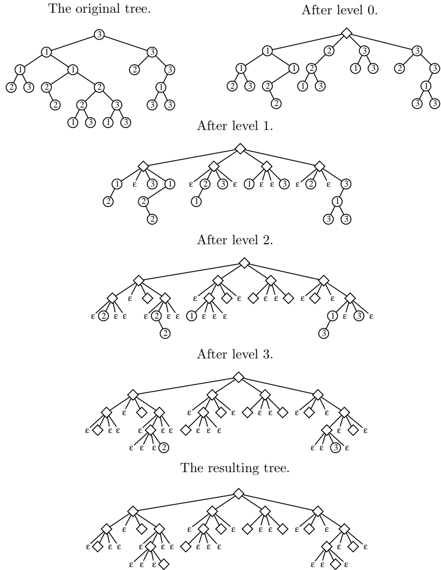
Figure 3. An illustrating example of the bijection presented between a \mathcal{Q}_{\geq 0} -free 3-coloured binary tree of size 21 and a 4-ary tree of the same size. The recursive procedure is here performed level by level, where, for better readability, the nodes in the resulting uncoloured 4-ary tree are drawn as diamonds. We have omitted the empty subtrees \varepsilon in the original tree as well as for the leaves of the resulting tree.
