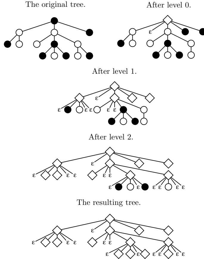
Figure 2. An illustrating example of the bijection presented between a black-rooted \bullet_0 -free two-coloured ternary tree of size 14 and a 5-ary tree of the same size. The recursive procedure is here performed level by level, where, for better readability, the nodes in the resulting uncoloured 5-ary tree are drawn as diamonds. We have omitted the empty subtrees \varepsilon in the original tree as well as for the leaves of the resulting tree.
