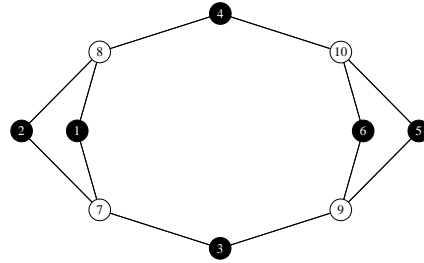
Figure 1. An \alpha -Kuramoto partition with two parts.
