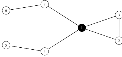
Figure 3. A graph G with a partition of V(G) into \{1\} and \{2, \dots, 7\} satisfying condition 2 in Theorem 2. This is the graph in Figure 1a of [5].
