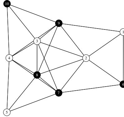
Figure 2. A graph G with a partition of V(G) into \{1, \dots, 5\} and \{6, \dots, 10\} satisfying condition 2 in Theorem 2.
